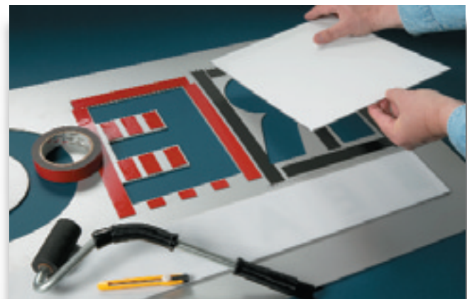
Easily cut to size, 3M™ VHB™ Tape 5952 bonds polycarbonate sheets to the back of a routed aluminum face. Surface is simply cleaned prior to application. Tape is pressed with a roller for optimum bonding.
